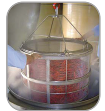
• BLANCHING TANK
