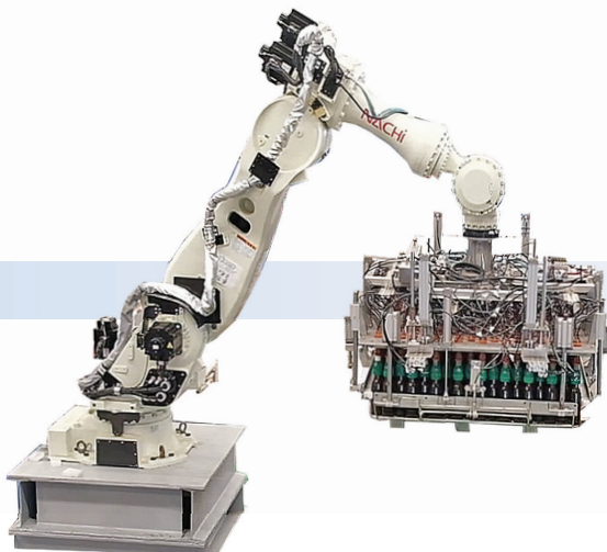
• ROBOTIC PALLETIZER AND CONVEYOR SYSTEM FOR CARTON BOX
